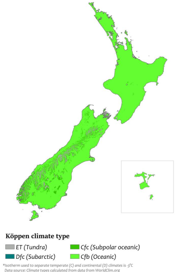
Köppen climate types of New Zealand
